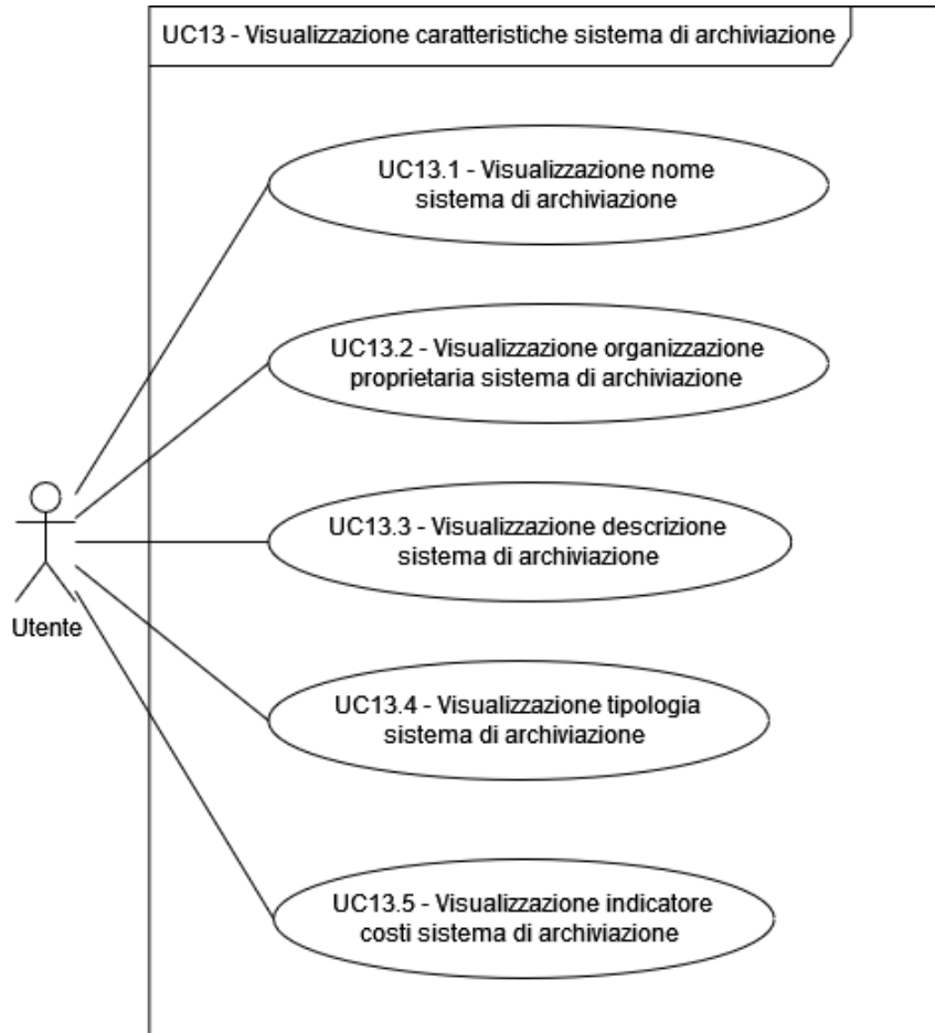
Figura 14: Diagramma UC13
